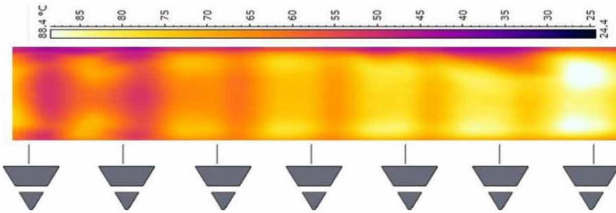
(b) Re=5431 (L2)
