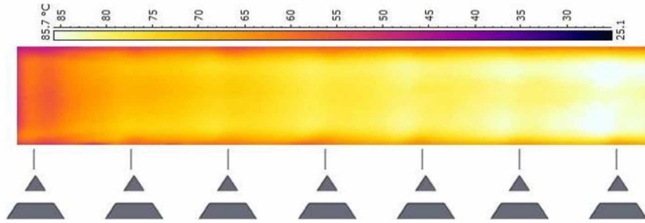
(b) Re=5431 (N2)
