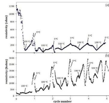
Figure 8: Variation of resistivity throughout heating-cooling system in the range 0-100 °C for (a): POT and (b): PKC including 29.4% POT.
