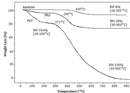
Figure 6: TGA curves of kaolinite, POT and PKC including 29.4% POT.
