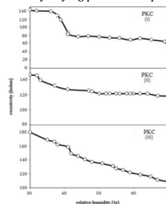
Figure 10: Variation of resistivity for PKC including 29.4% POT in 30-70% humidity range during humidify-drying processes repeated three times.
