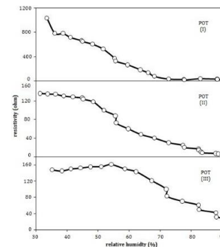
Figure 9: Variation of resistivity for POT in 30-90% humidity range during humidify-drying processes repeated three times.
