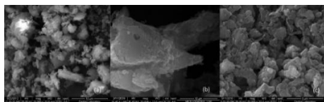
Figure 7: SEM micrographs of (a): Kaolinite, (b): POT and (c): PKC including 29.4% POT.
