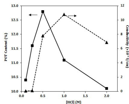
Figure 1: The influence of HCl concentration on (■) POT content and (▲) Conductivity of PKC ([APS]: 0.07 M, [o-toluidine]: 0.1 M, polymerization time: 2 h, temperature: 20 ^{\circ}\text{C} ).
